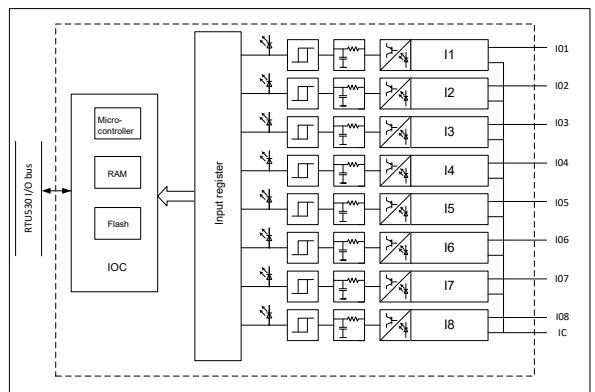
Figure 2: Block diagram binary input unit
