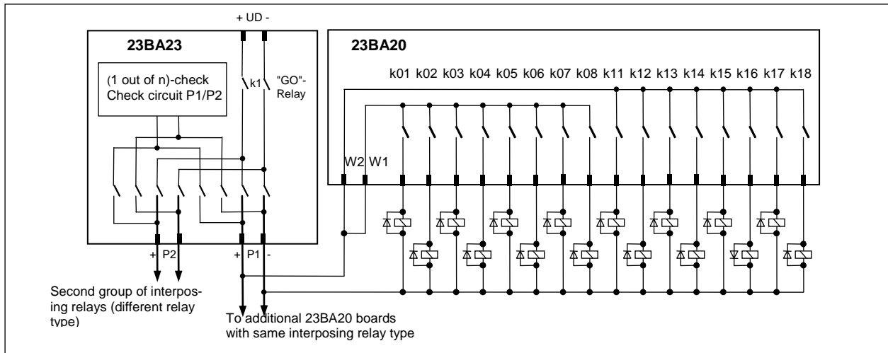
Fig. 3 :-Block diagram: Object command output with (1 out of n) check (1 out of n) check at 1.5 pole connection
