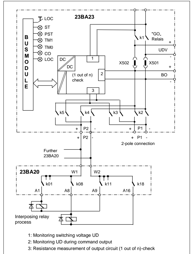
Fig. 1: Function block diagram 23BA23
