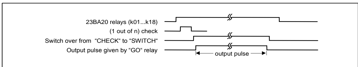
Fig. 5: Timing diagram of command output: Coordination of 23BA23 and 23BA20 by communication unit
