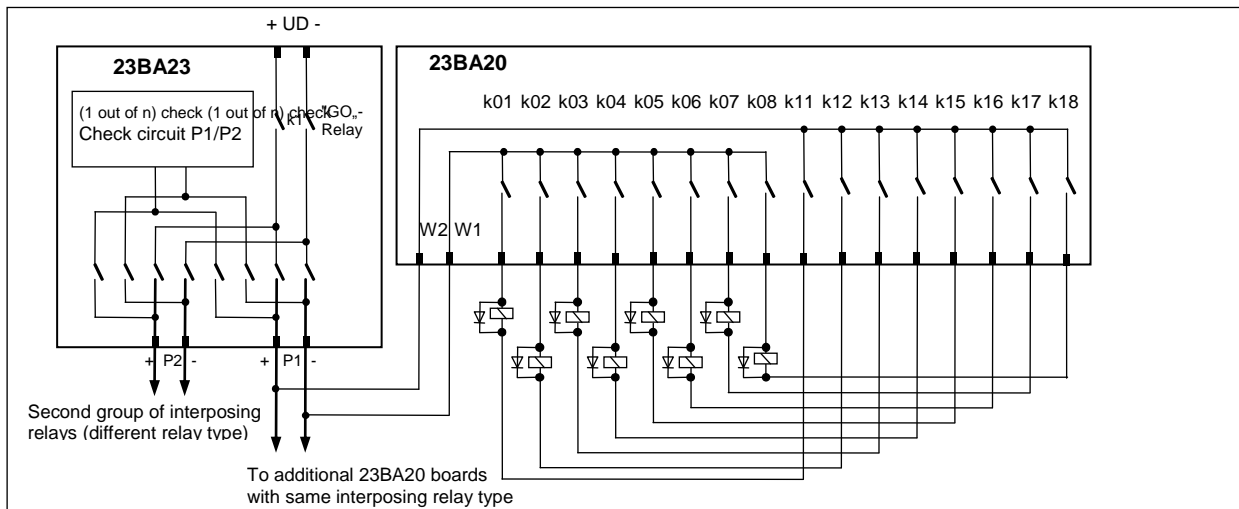
Fig. 4: Block diagram: Object command output with (1 out of n) check (1 out of n) check at 2 pole connection
