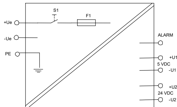
Figure 1: Block diagram 560PSU01
